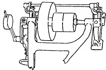
FIG. 134. SWING CUT-OFF SAW WALL HANGERS.
